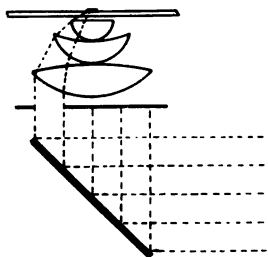
Fig. 54. Illuminating object by oblique light with condenser.
